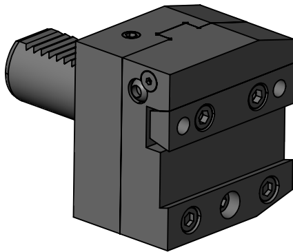
90DEG VDI30 STATIC TOOL OUTPUT: 26mm BLADE COOLANT: EXTERNAL
